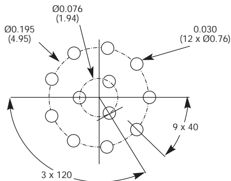
PCB Cutout (D Termination)
